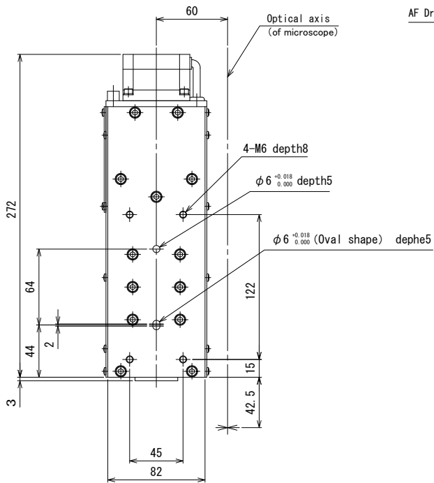
Drive unit installation drawing
