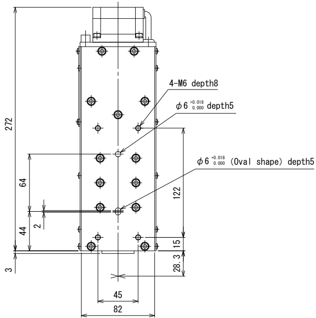
Drive unit installation drawing
