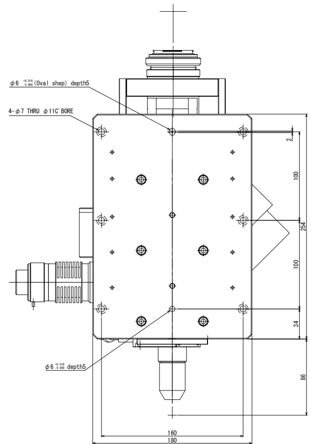
Installation drawing
