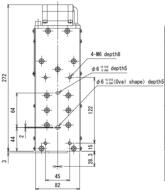
Drive unit installation drawing
