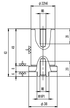
Shank \phi 32 detail view
